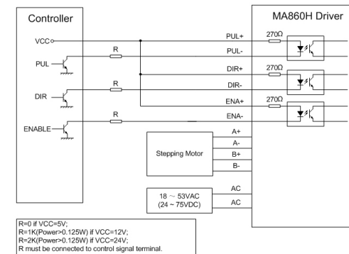
Figure 10: Typical connection
